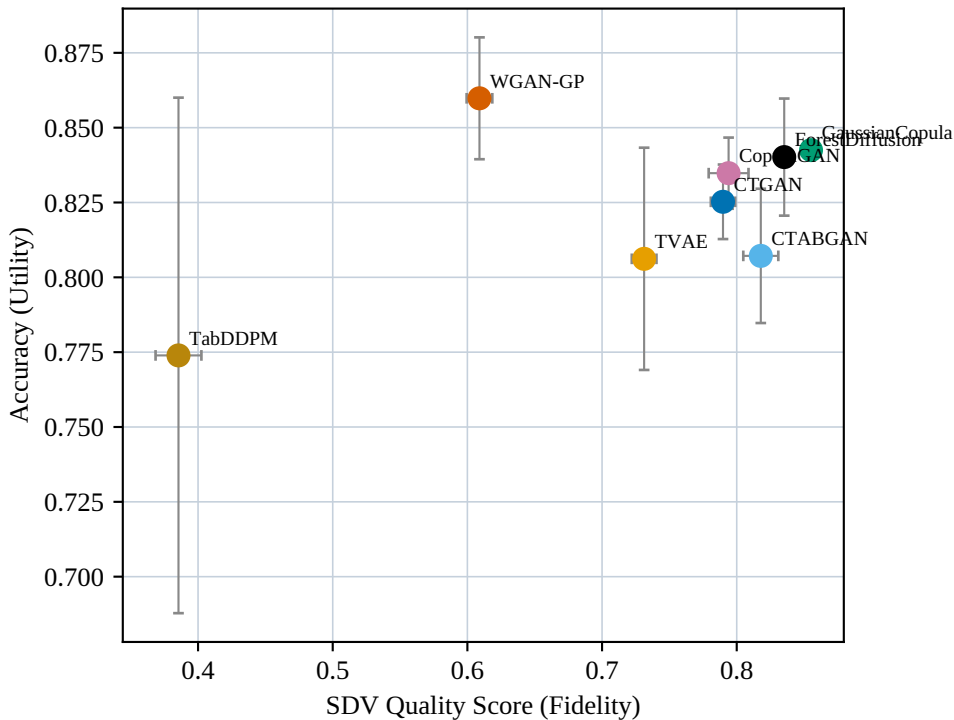
Bank Marketing: SDV Quality Score (Fidelity) vs Accuracy (Utility)
